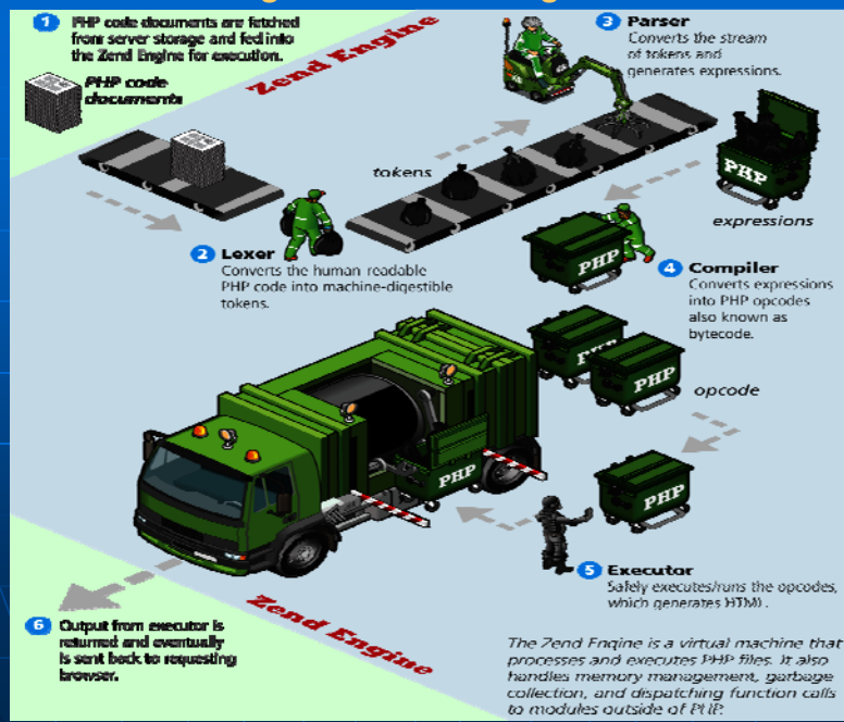
Figure 8.8 Zend Engine
