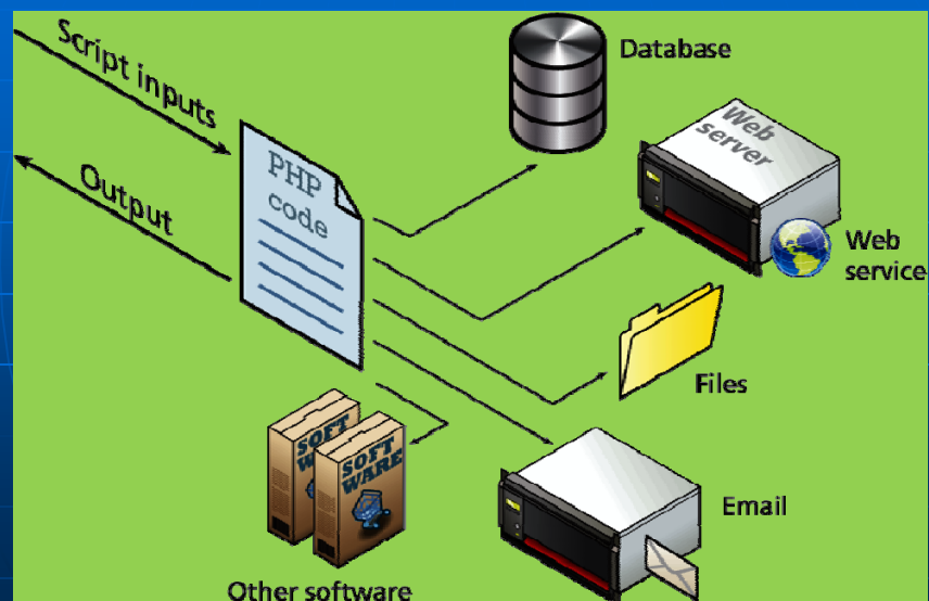
Figure 8.2 Accessible Resources for Server Scripts
