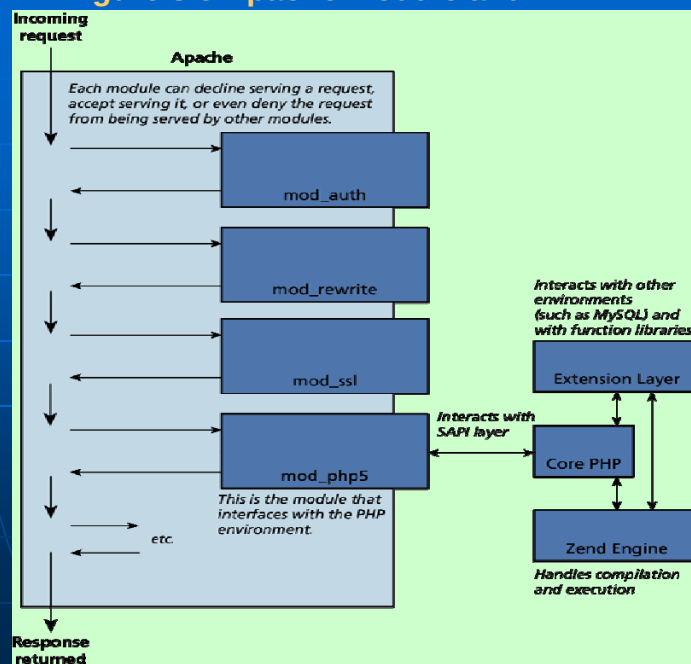
Figure 8.6 Apache Module and PHP
