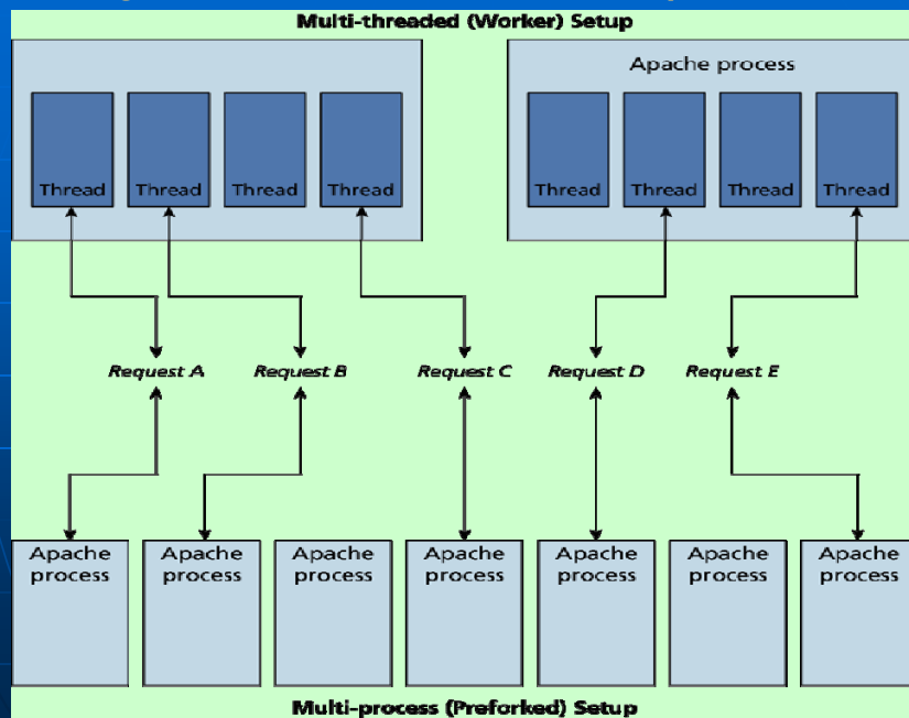
Figure 8.7 Multi-threaded vs. Multi-process
