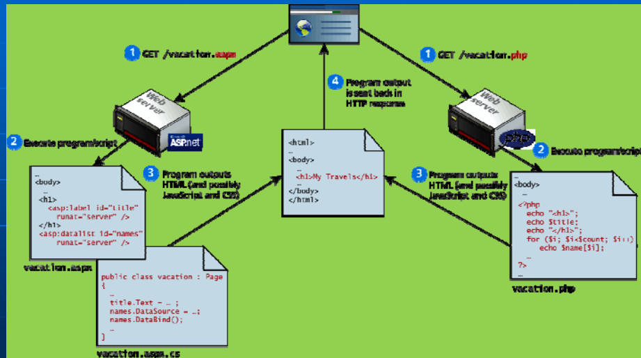
Figure 8.3 Web Development Technologies
