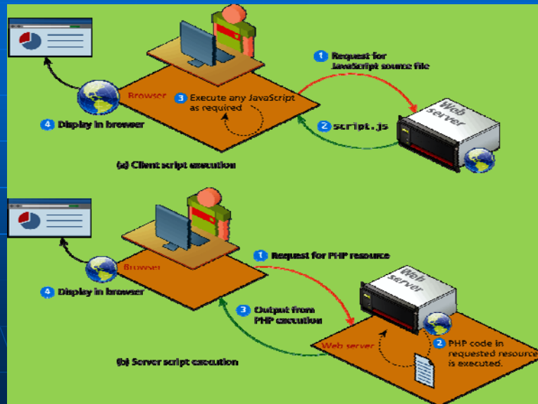
Figure 8.1 Server-Side Script vs. Client Side Script
