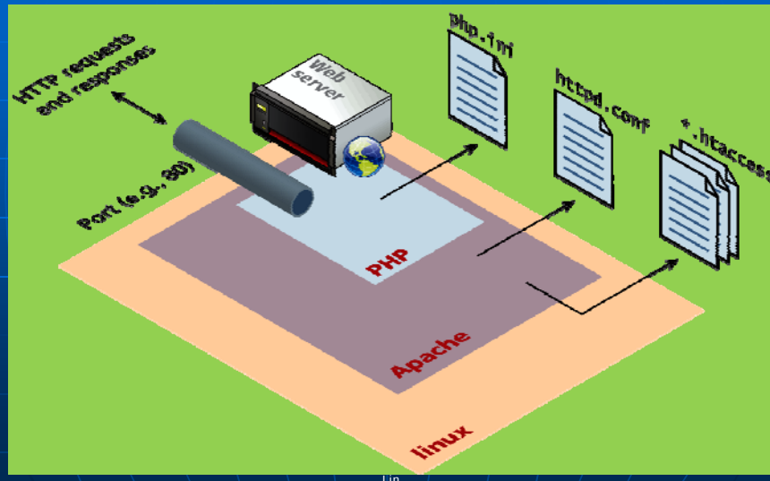
Figure 8.5 Linux, Apache, and PHP
